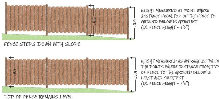
Figure 3-03. Fence Height
