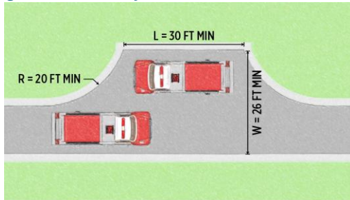
Figure 3-02. Driveway Pull-Offs
